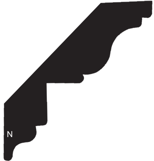
P 141 3/4" x 3 5/8"
